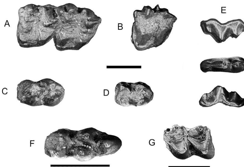
Fig. 6. The ruminants of Chaungtha. A–E: cf. Siamotragulus sp.. A, left M1/-M2/ or M2/-M3/ CTA 51-1 in occlusal view; B, left upper molar CTA 51-2 in occlusal view; C, left M1/ or M2 CTA 51-3 (occlusal view); D left M1/ or M2 CTA 51-4 (occlusal view); E, right P3 CTA 51-5 in lingual, occlusal and labial view (from top to bottom); F, right M3 of cf. Siamotragulus sanyathanai ; G, right M1/ or M2 of ?Bovidae indet. in occlusal view. Scale bars: 1 cm.
