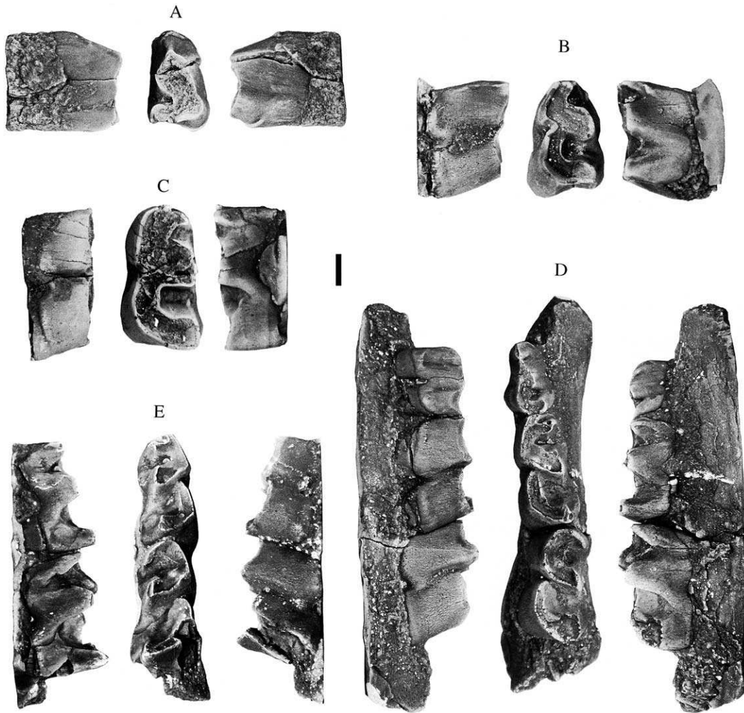
Fig. 3. The rhinocerotids of Chaungtha. A, B and C: Brachypotherium fatehjangense . A, right P/2 CTA 55-1; B (in lingual, occlusal and labial views); left P/3 CTA 55-2 (in lingual, occlusal and labial views); C, left dP/3 CTA 55-3 (in lingual, occlusal and labial views). D and E: Rhinocerotidae indet.. D, left series with dP/2–dP/4 CTA 54-1 (in lingual, occlusal and labial views); E, right series with dP/3–dP/4 CTA 54-2 (in lingual, occlusal and labial views), from the same individual as CTA 54-1. Scale bar: 1 cm.
