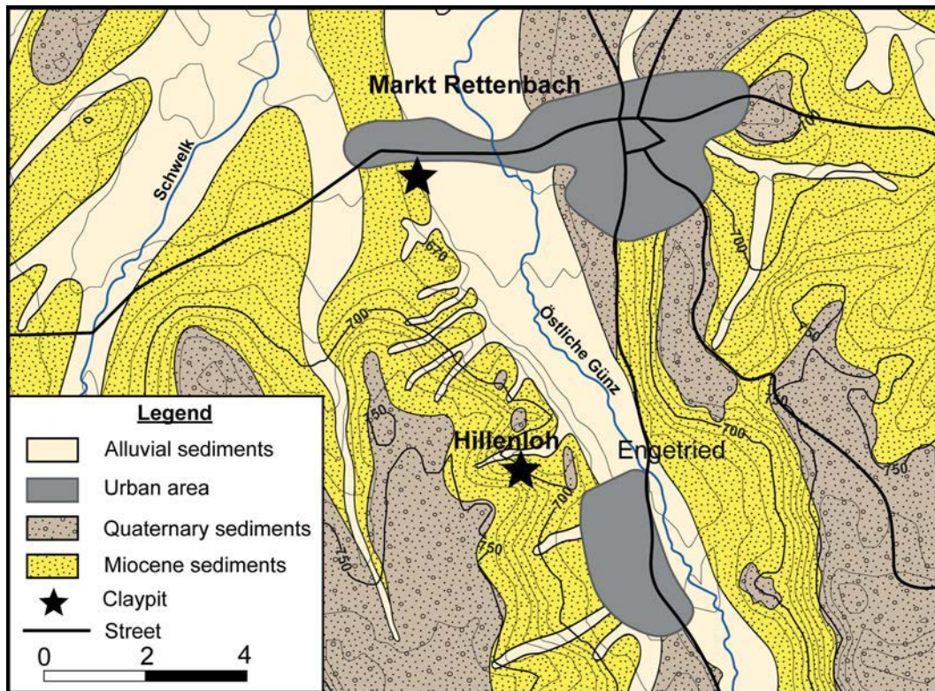
Fig. 2. Geological map of the study area (see Fig. 1) after SCHÄFER & BERLINGER (1954: 22). The topography was generated with GMT6 (WESSEL et al. 2013). The black stars indicate the fossil localities Markt Rettenbach and Hillenloh.
