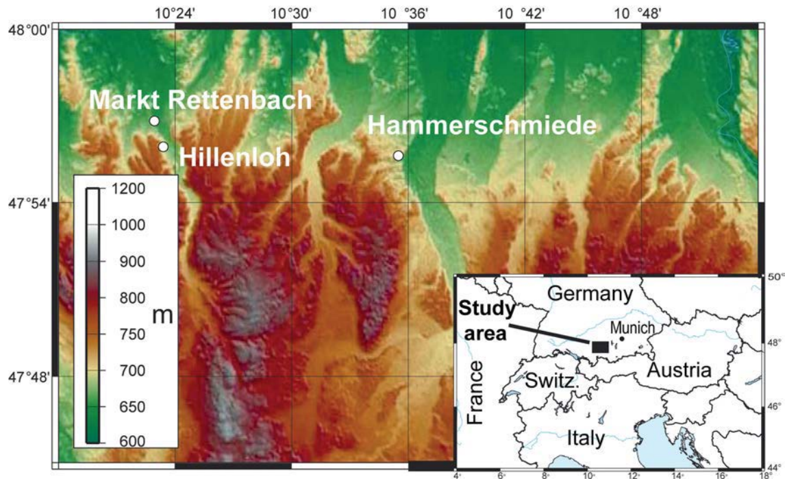
Fig. 1. Topographic map of southwestern Bavaria (Germany), indicating the position of the Middle and Late Miocene localities Markt Rettenbach, Hillenloh, and Hammerschmiede in the area. The map was made with GMT6 (Wessel et al. 2013).
