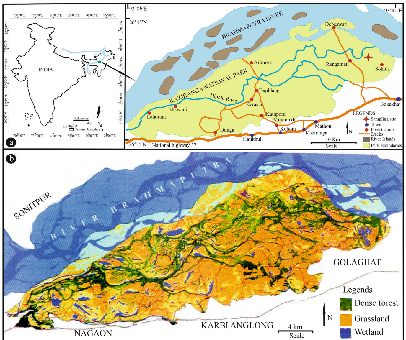
Fig. 1. a. Location map of the sampling site, b. Vegetation coverage map of the Kaziranga National Park (after Das et al., 2014).
