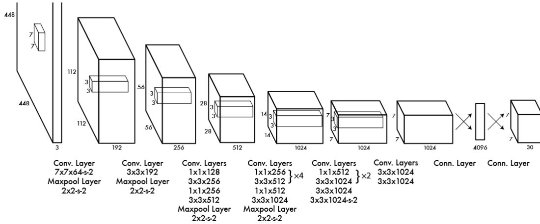
Figure 5: Model architecture of the original YOLO model [18]
