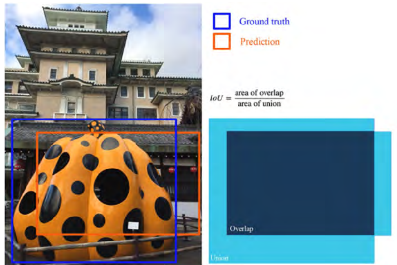
Figure 7: IoU visualized [22]
