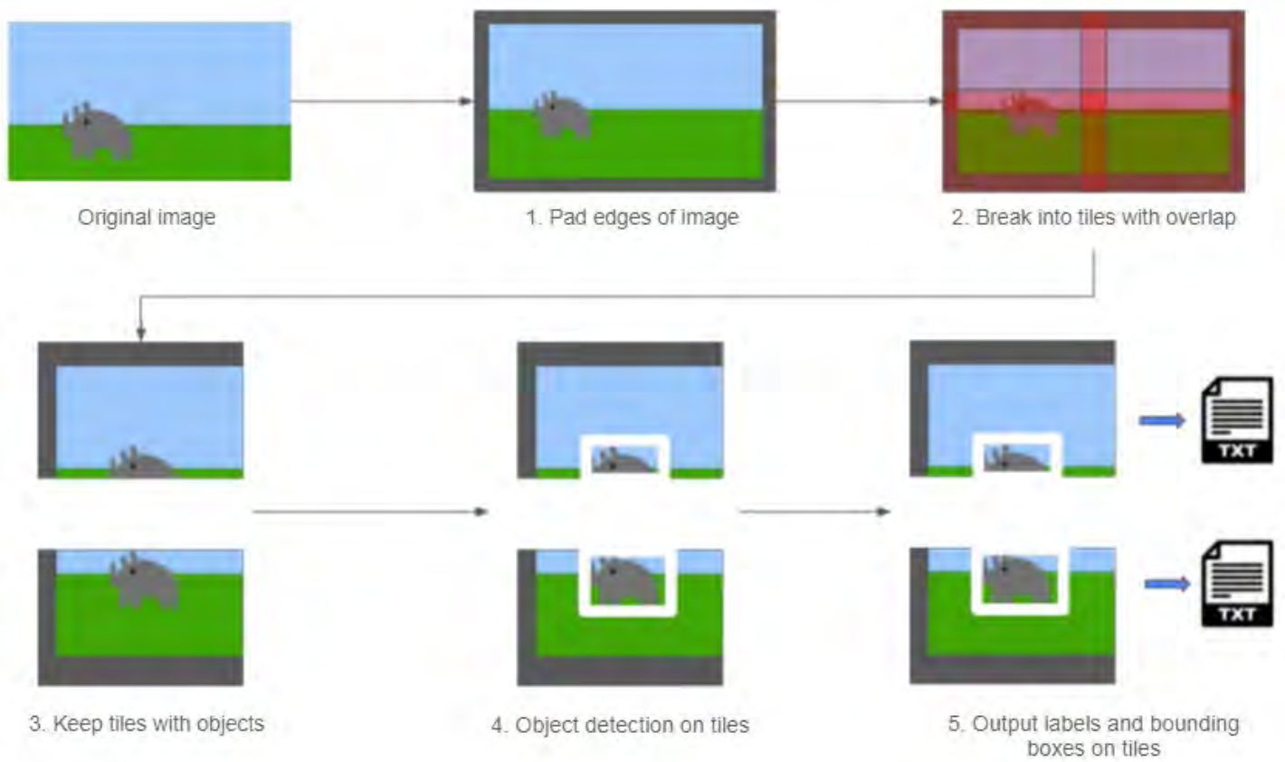
Figure 12: Step by step tiling process
