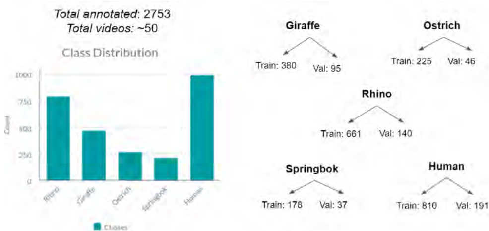
Figure 3: Classes and distribution into train and validation sets
