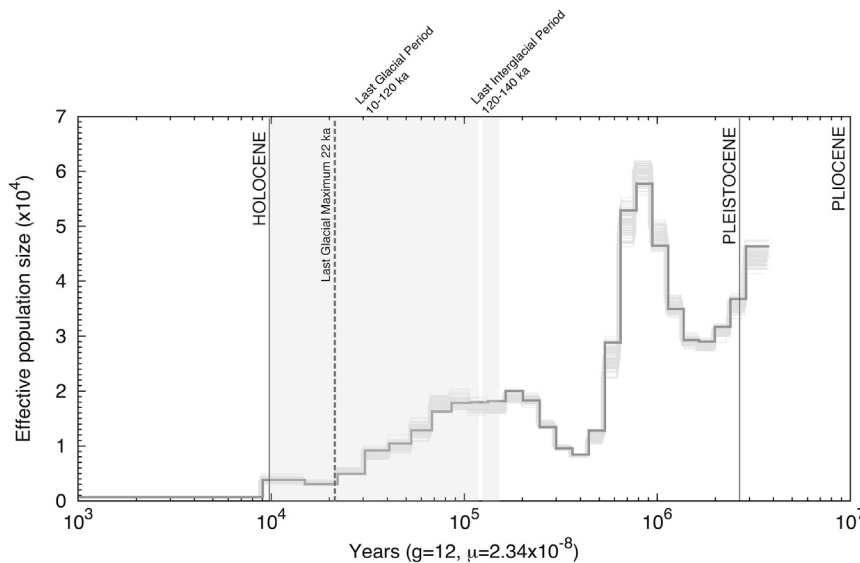
Figure 1. Demographic History of the Sumatran Rhinoceros
