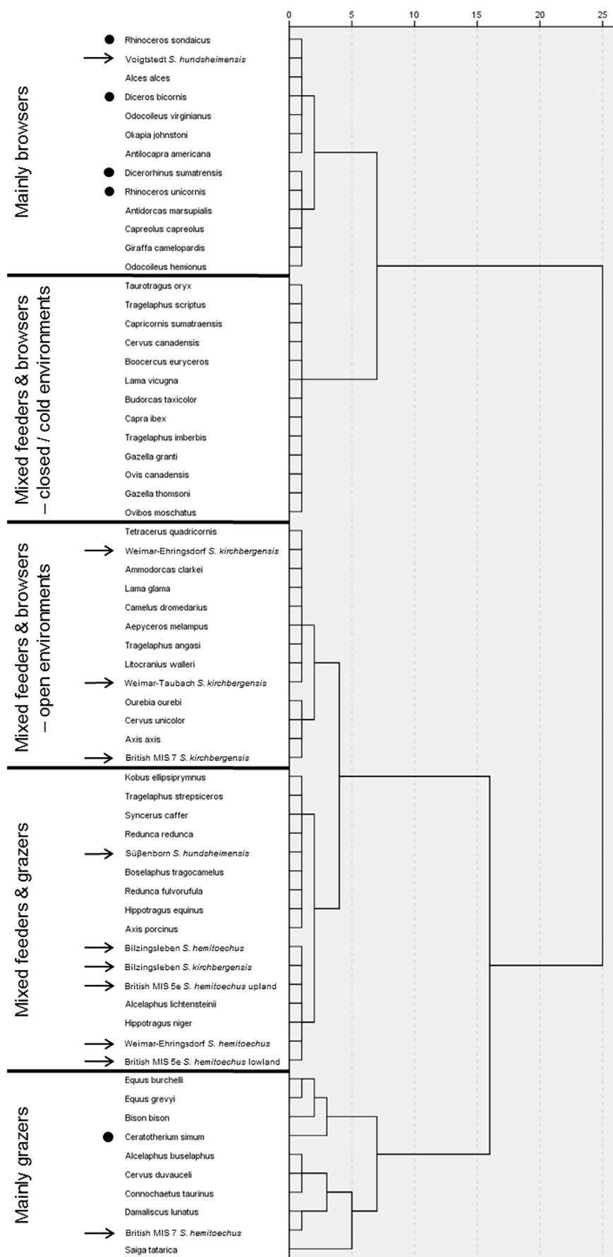
Fig. 7. Cluster diagram using mesowear variables for extant herbivores and European Pleistocene rhinoceros assemblages; dots: extant rhinoceros species; arrows: Pleistocene samples.
