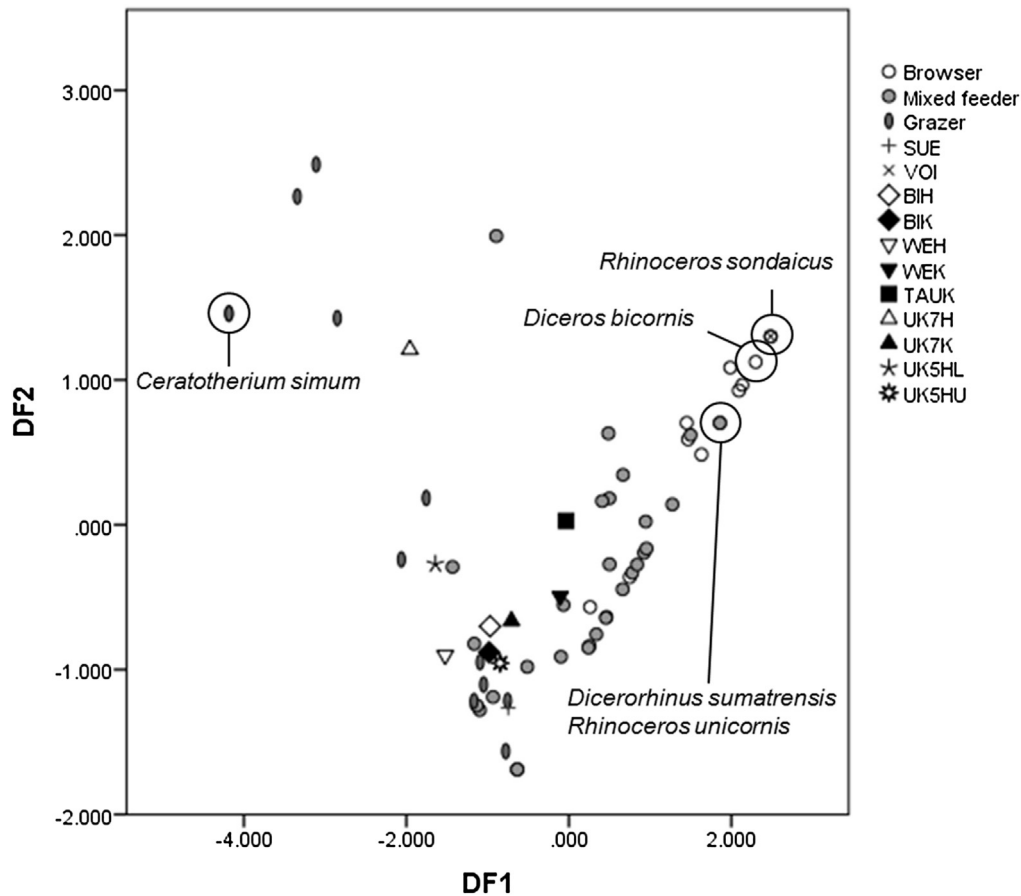
Fig. 6. Plot of scores on DF2 vs. DF1 for a range of extant herbivore species and Pleistocene rhinoceros assemblages; abbreviations: see Table 1.
