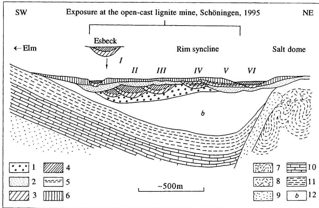
Figure 2. Schematic section through the Quaternary sedimentary sequence in the depression along the Stassfurt-Helmstedter salt dome, showing the channels I to VI.
