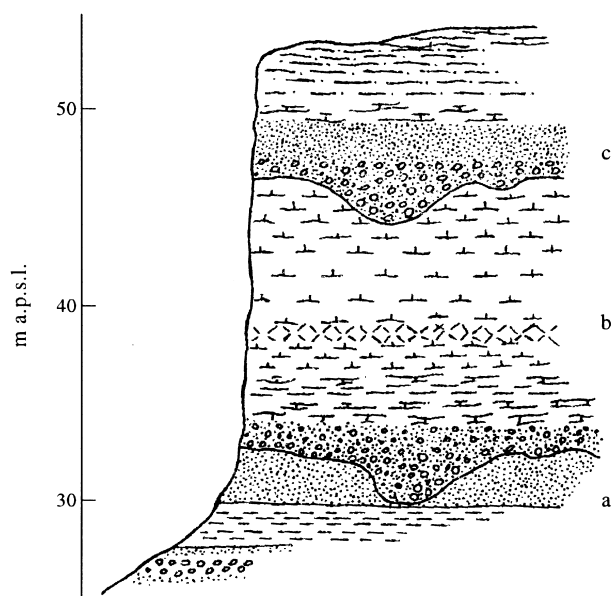
FIG. 2. The Torre del Pagliaccetto section: (a) Sicilian sediments; (b) Aurelia formation; (c) II sedimentary cycle of Torre del Pagliaccetto (redrawn and modified from Malatesta, 1978).
