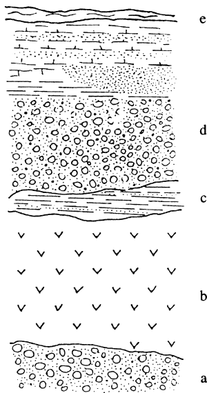
FIG. 4. The Sedia del Diavolo section: (a) I sedimentary cycle consisting of gravels and sands with volcanic minerals (San Cosimato formation); (b) Tufo litoide lionato ; (c) II sedimentary cycle consisting of clays and silts (Aurelia Formation); (d) gravels and sands, clays, epivolcanites, marls and travertines of the III sedimentary cycle (Vitinia formation). (N.B. The drawing of this section, which is now no longer exposed, lacks an altitude scale, since this information is missing on the manuscript diagram by A.C. Blanc, from which this figure has been redrawn).
