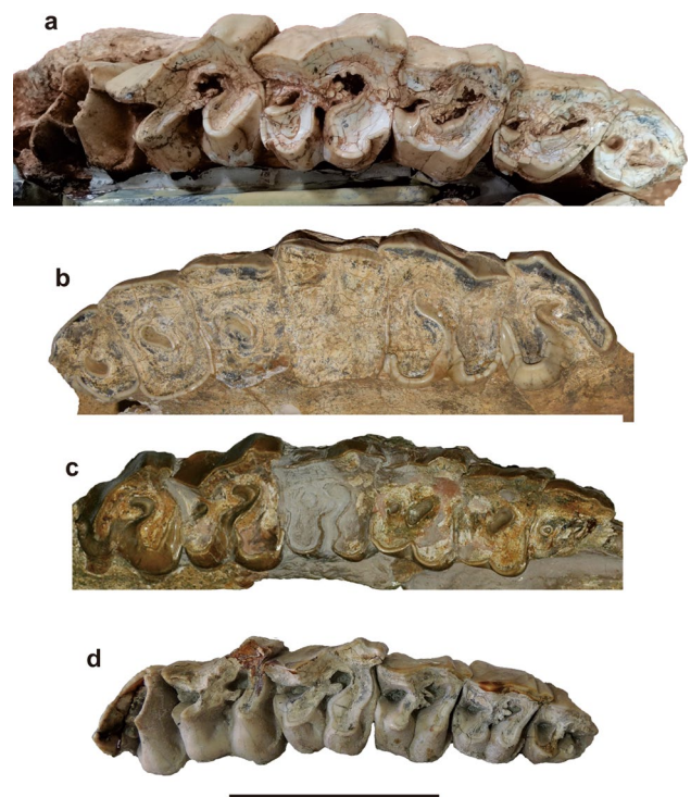
Fig. 6 Comparison of Pliorhinus upper teeth. a-b. Pliorhinus ringstroemi a. HMV2048, right P2-M3; b. HMV1115, left P2-M3; c. Pliorhinus megarhinus from Baccinello (NMB BAC n.c, right P2-M3; image from Pandolfi and Rook 2017); d. Pliorhinus miguelcrusafonti from Kvabebi (GNM1 29-2013/925 DN-229, right P2-M3; image from Pandolfi et al. 2021). Scale bar equals 10 cm
