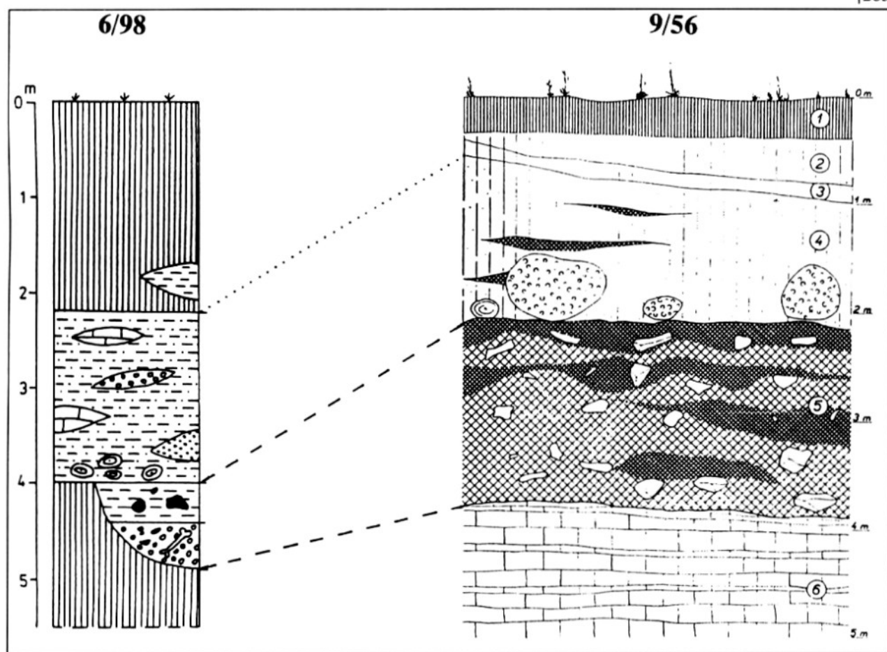
Fig. 7. The schematic comparison of the profile of pit 9/56 (Fejfar, 1964) with the profile of new pit 6/98.
