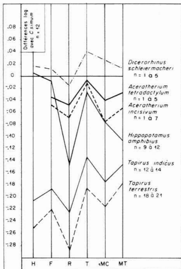
Ratio-diagrams of limb bones lengths in some aquaphile mammals. Same abbreviations as in fig. 1 and 2.
